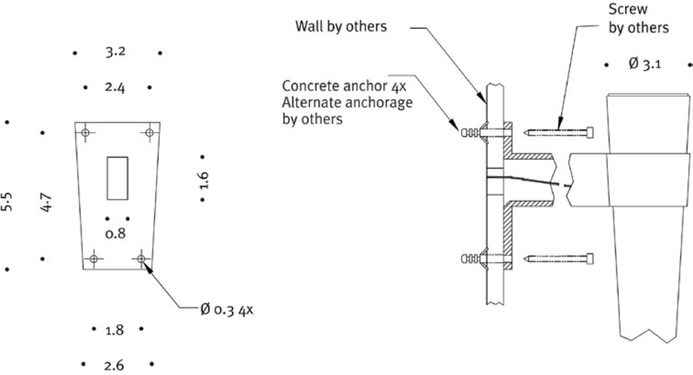
Standard Mounting
