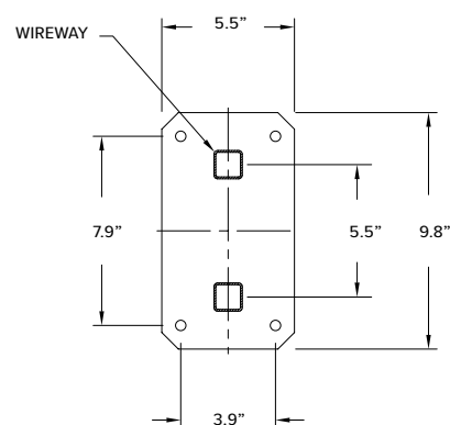
MOUNTING DETAIL
